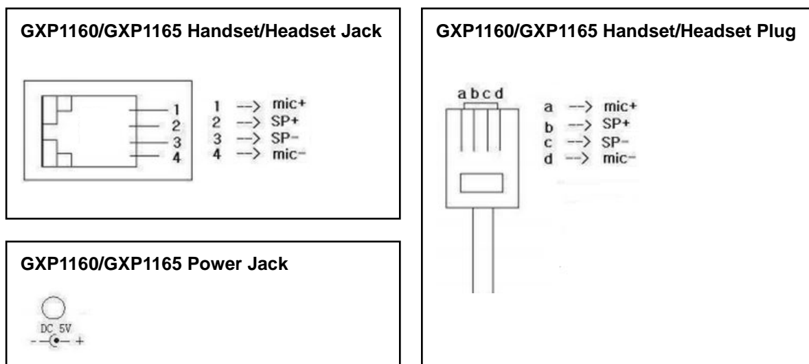
Figure 2: GXP1160/GXP1165 Pin-out
